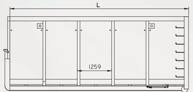
▲ MK 46 LP (LP - Logo plate version with a logo on the side wall)
