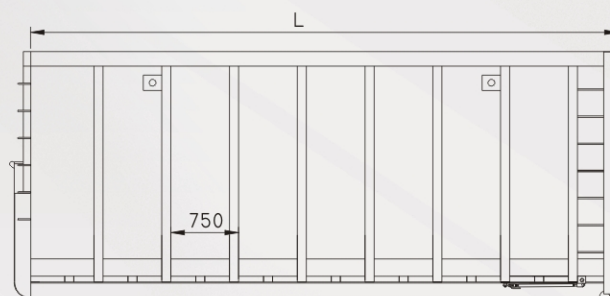
▲ MK 35MMH (MH - the roof is lifted by a hydraulic pump)
